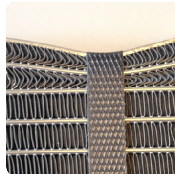
Top tubes bent by too tight strapping
